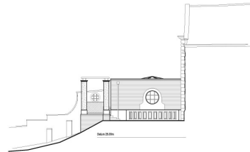
7 20 East Elevation Link Building
